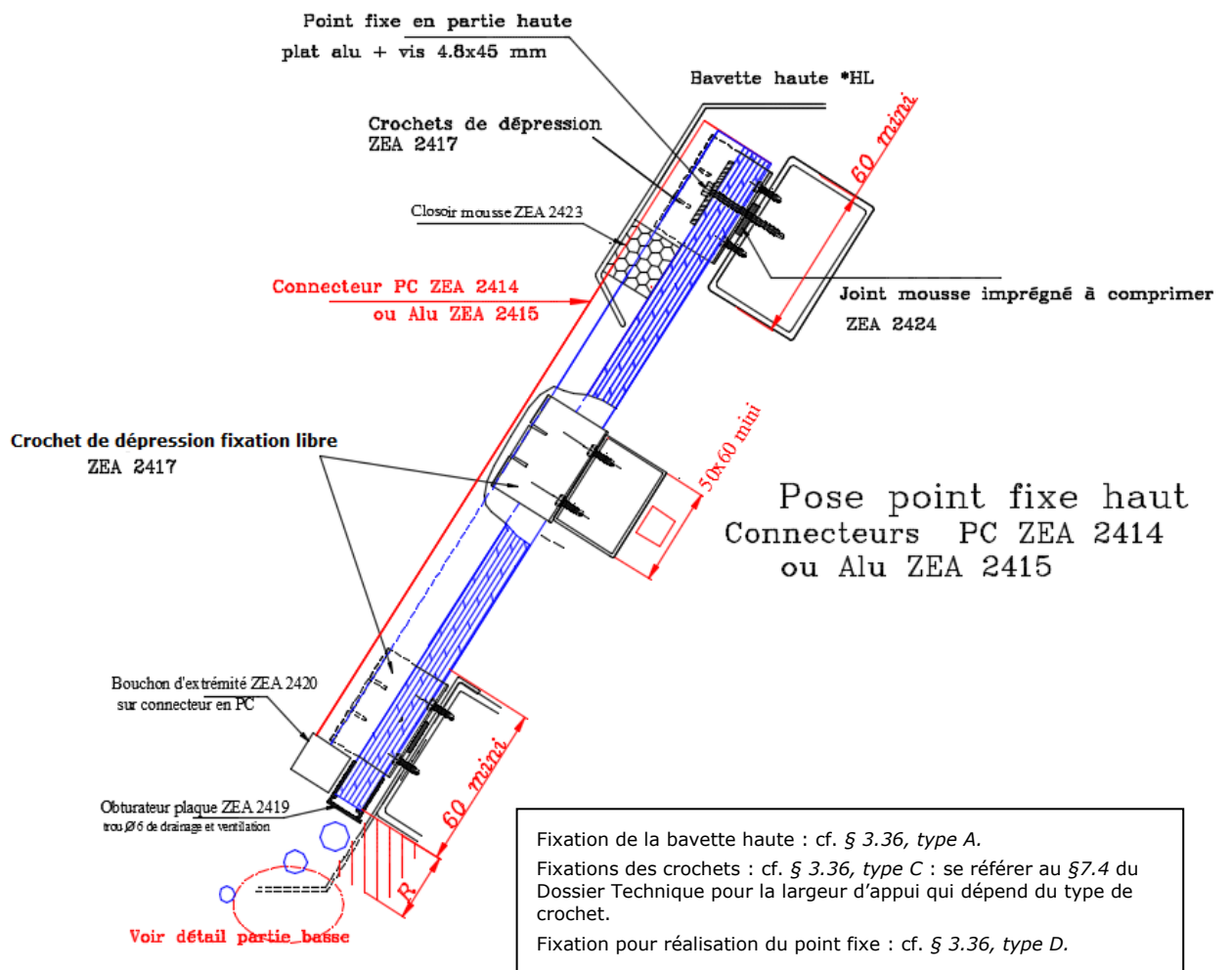
Figure 13 – Pose point fixe haut
