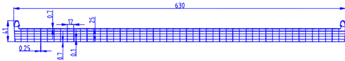
Figure 1b – Plaques AKYVER Connect®25
