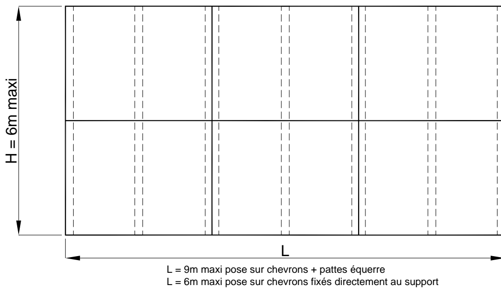
Figure 1bis – Pose jointive
