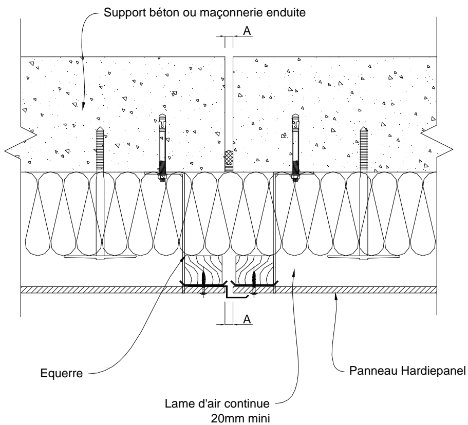
Figure 6bis – Joint de dilatation – Ossature bois
