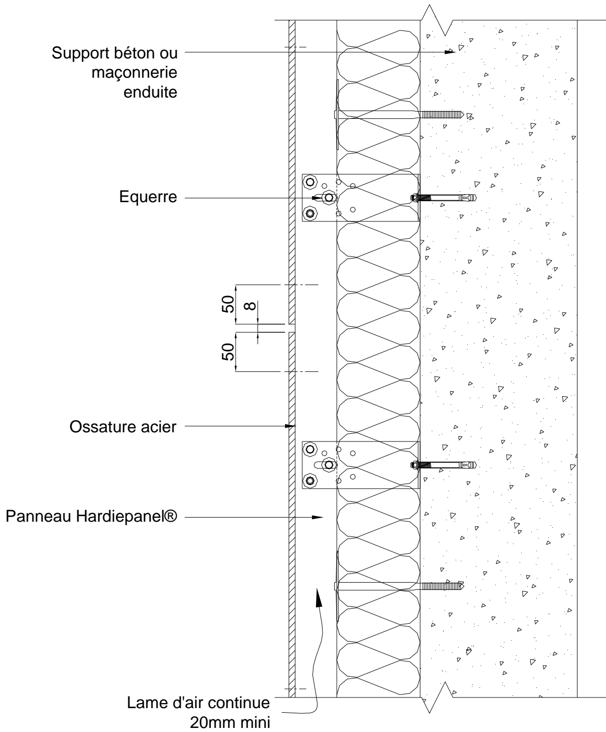
Figure 2 – Joint horizontal
