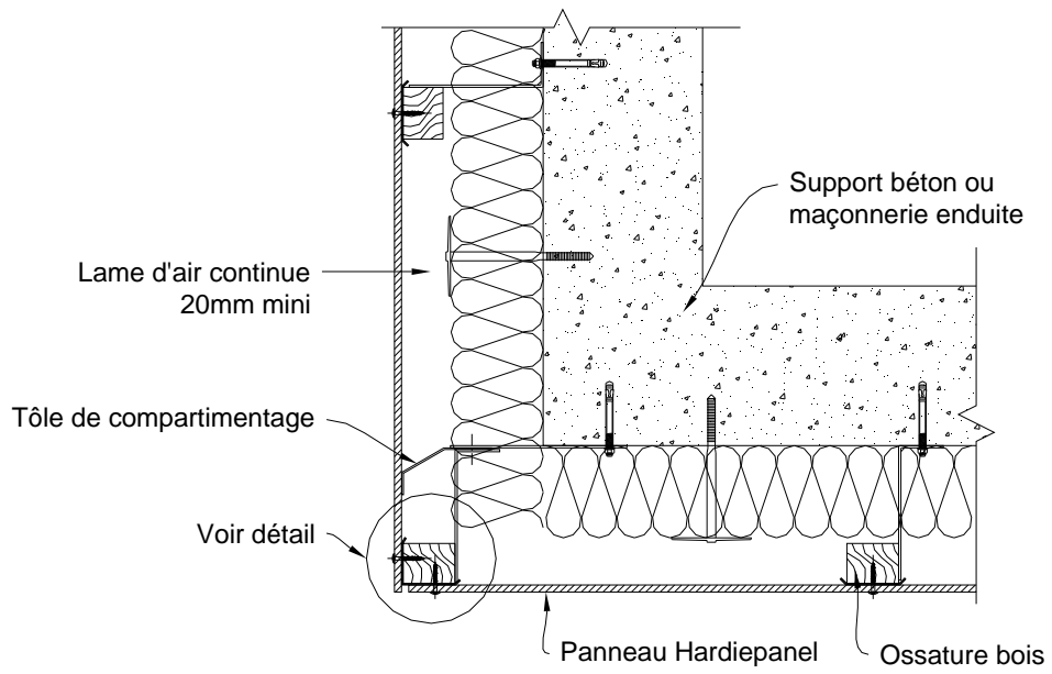
Figure 12 – Angle sortant
