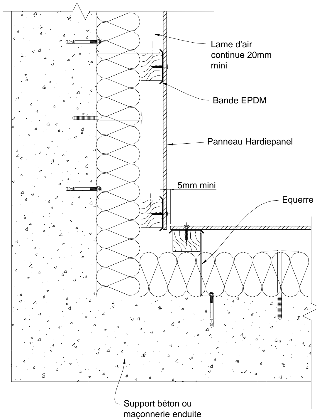
Figure 7 – Angle rentrant
