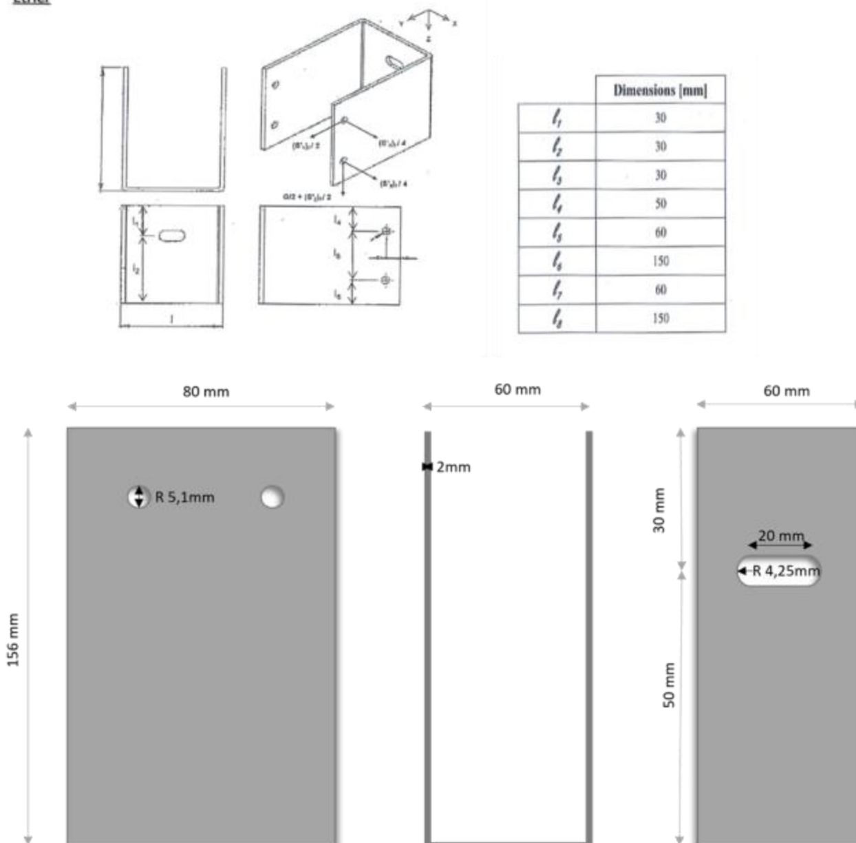
Figure A2b - Etrier (Tableau A1)
