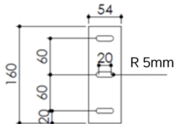
Figure A2a – Etrier (Tableau A2)
