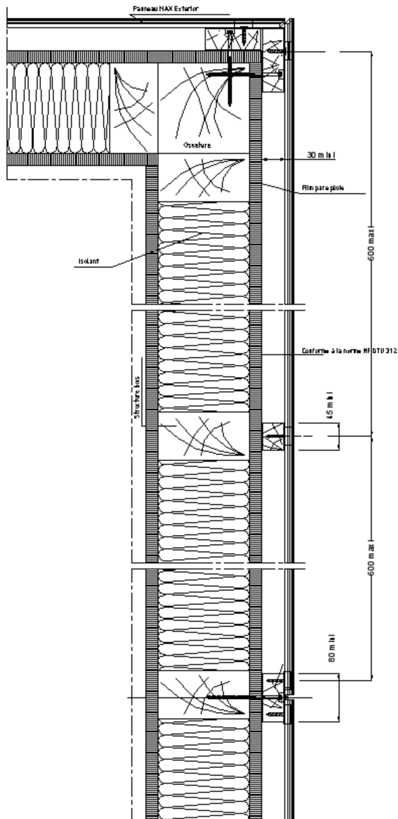
Figure A1 – Pose sur COB
