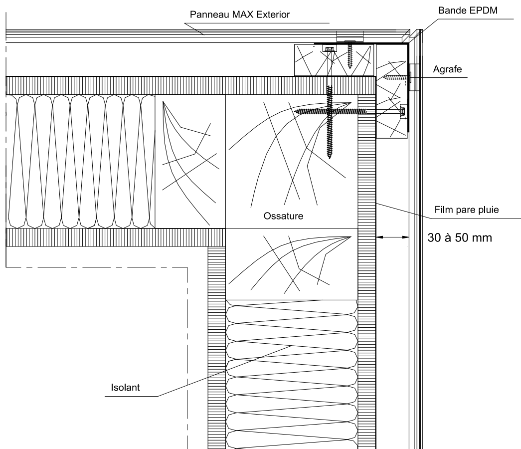
Figure A4 – Angle sortant – Pose sur COB
