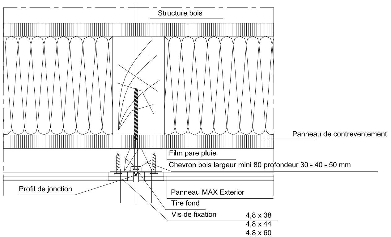
Figure A3 – Joint vertical de raccordement – Pose sur COB
