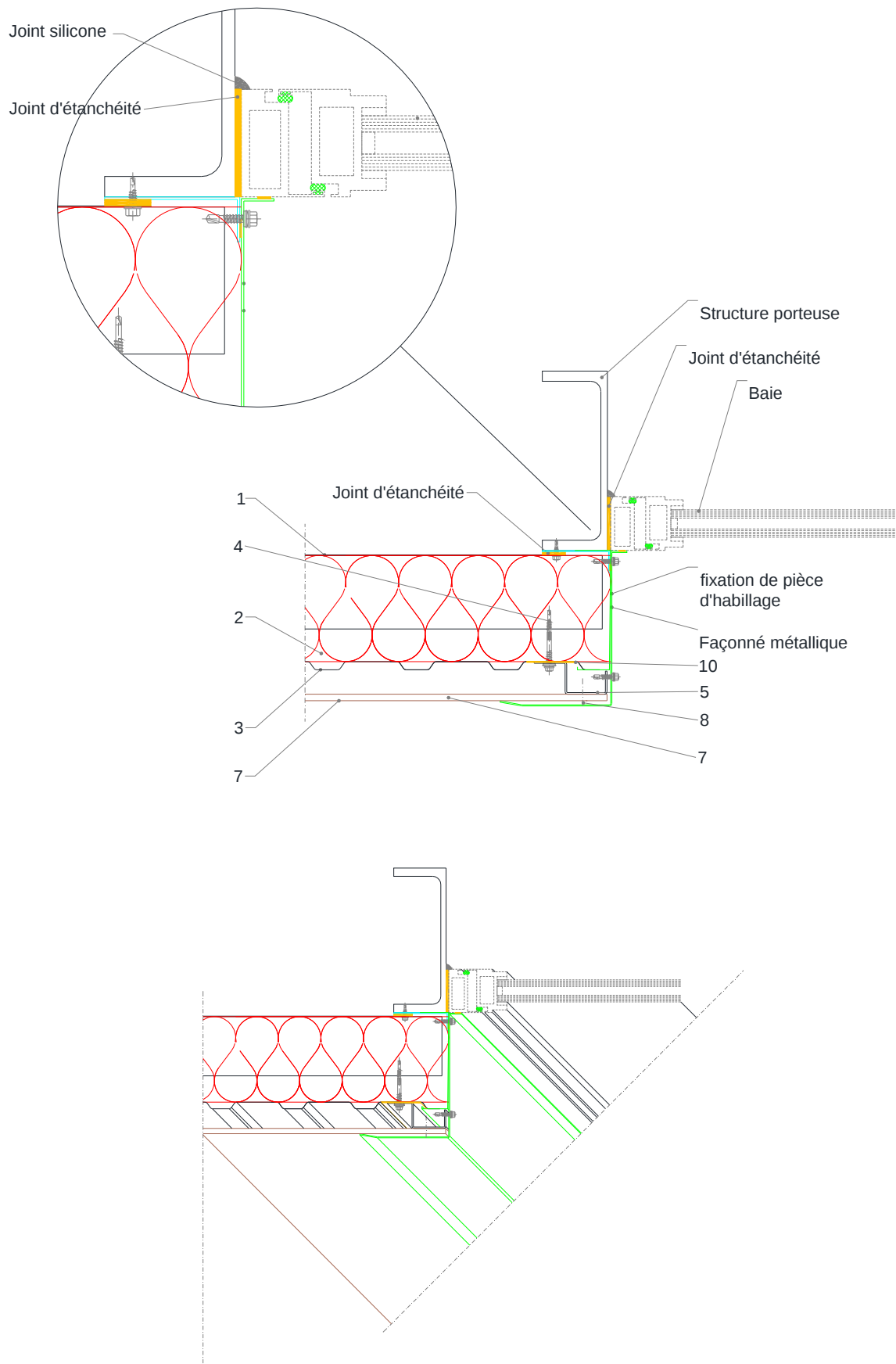
Figure 18 – Jambage – Coupe horizontale
