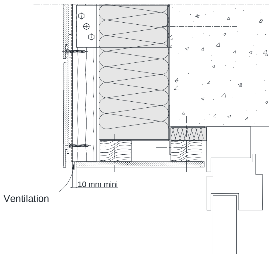
Figure 16 - Pose horizontale - Angle sortant
