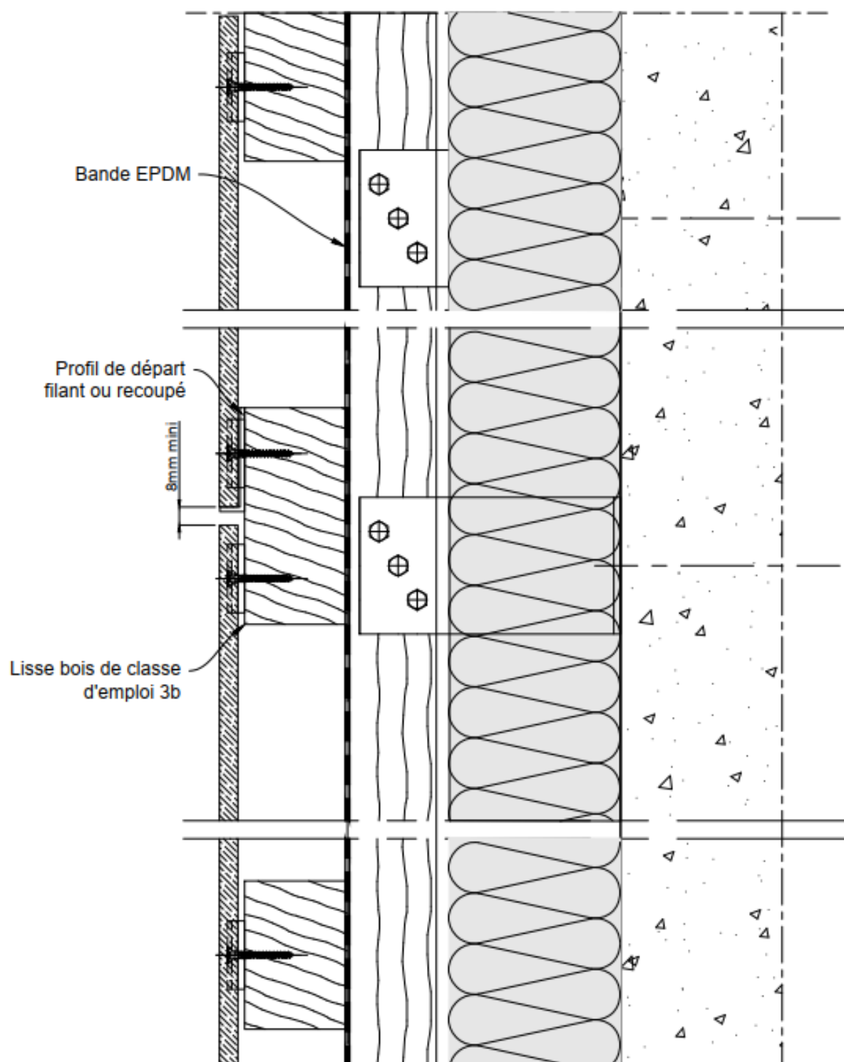
Figure 19 - Pose verticale – joint horizontal (coupe verticale)
