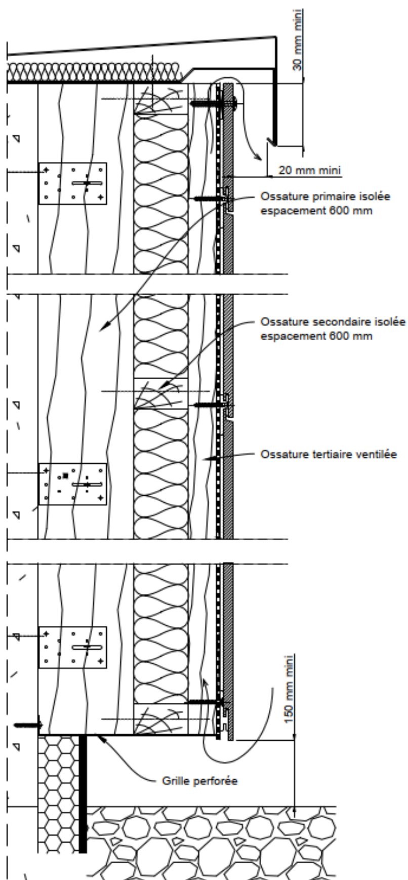
Figure 33 – Coupe verticale
