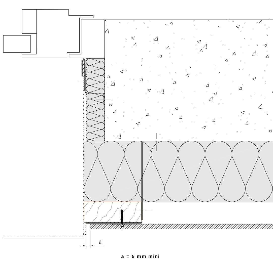
Figure 14 - Pose horizontale - Tableau
