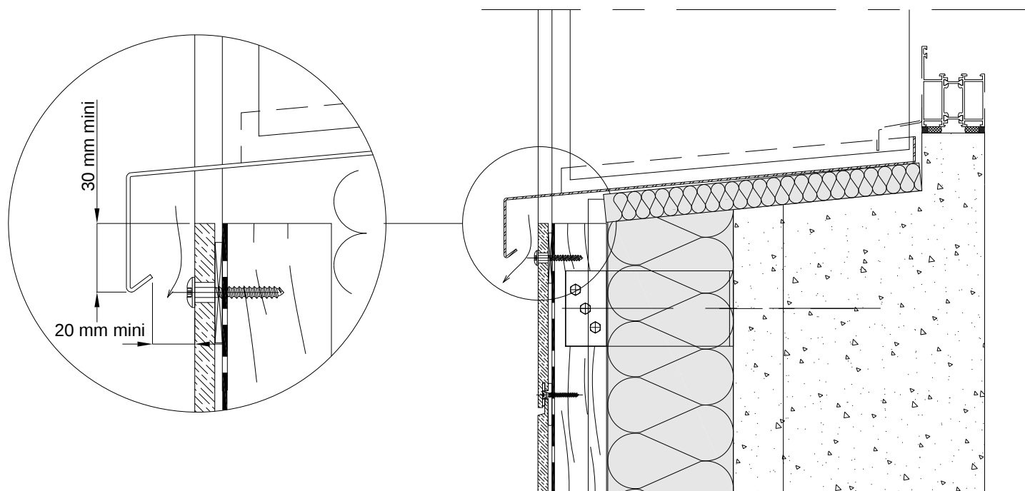
Figure 14 - Pose horizontale - Tableau
