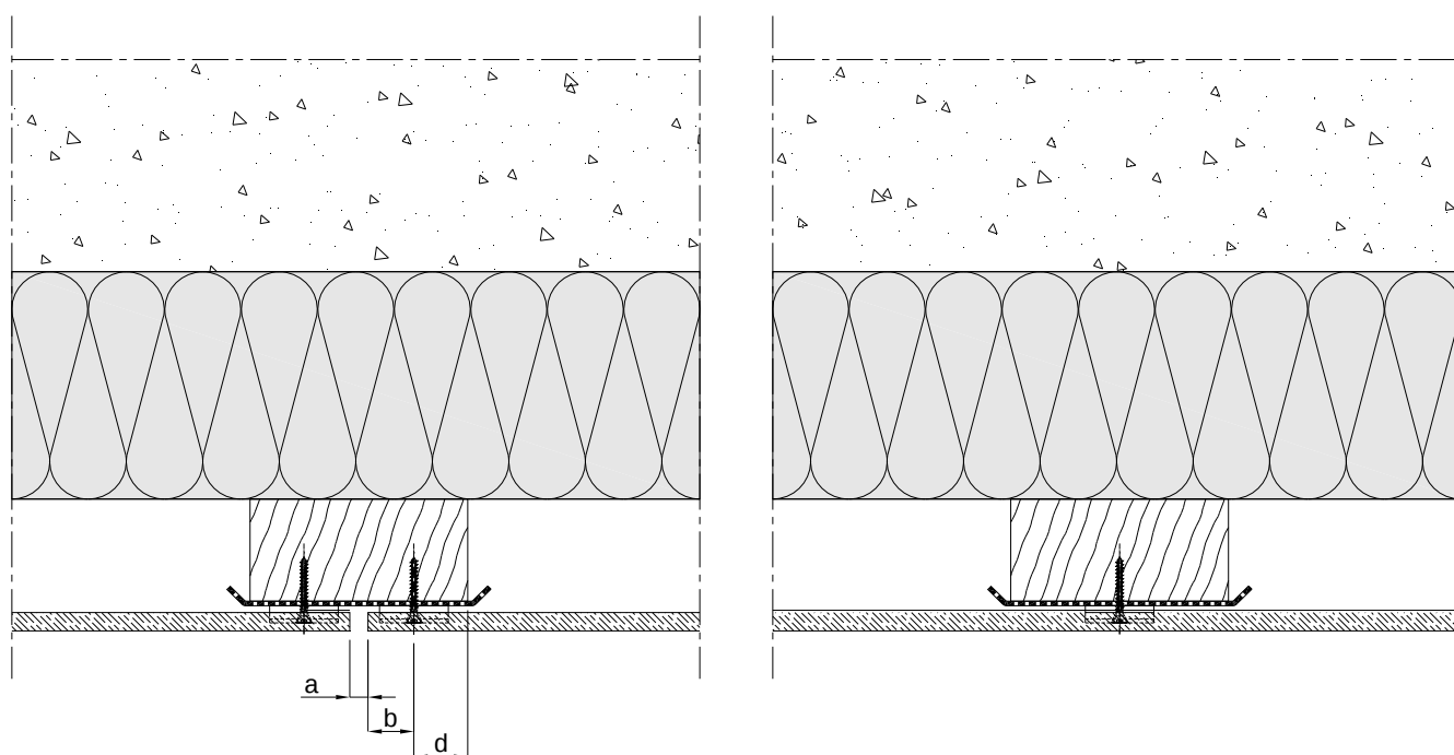
Figure 6 - Pose horizontale - Joint vertical (coupe horizontale)
