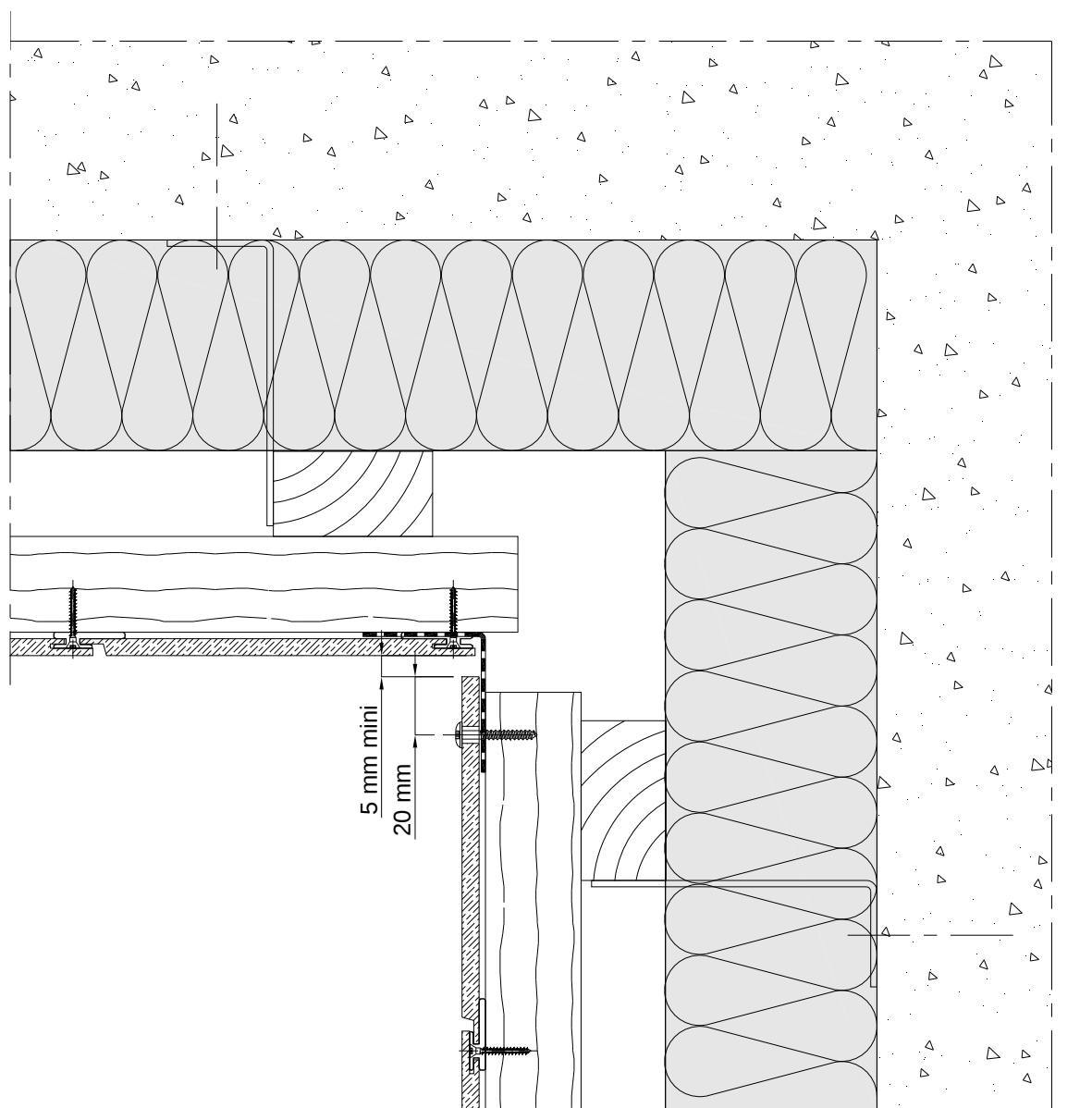
Figure 24 - Pose verticale - Angle rentrant
