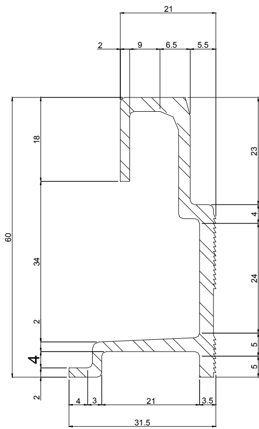
Figure 1 – Lisse TSP 203
