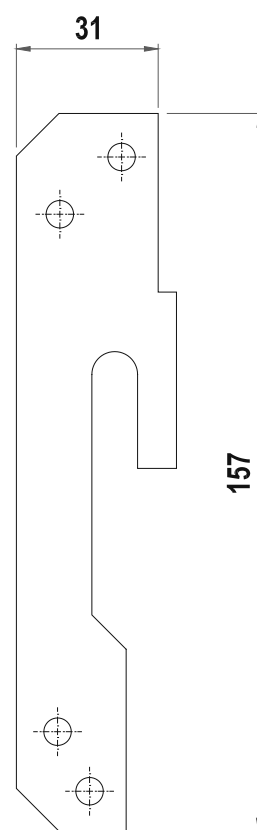
Figure 6bis – LCR-40
