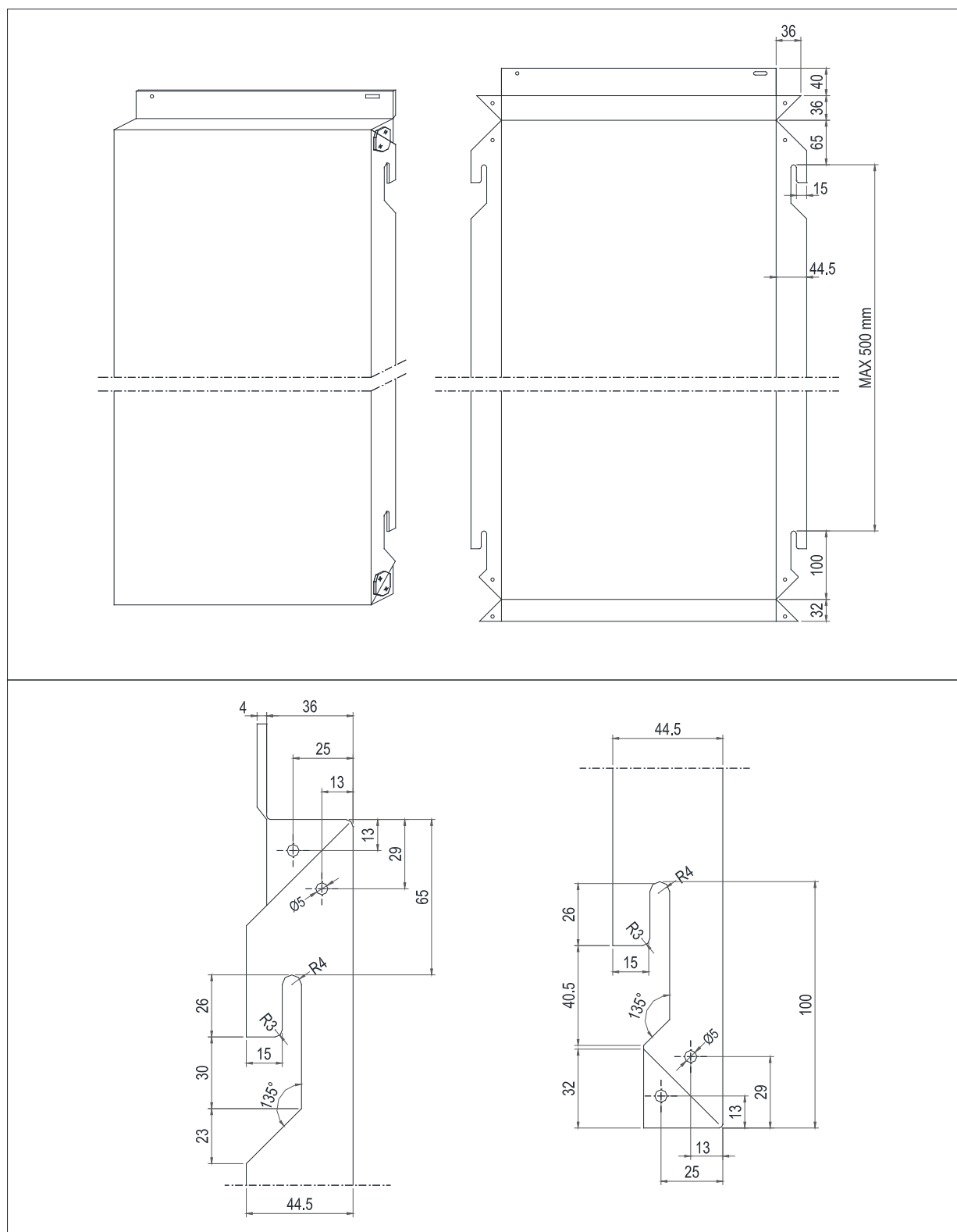
Figure 2 – Cassette
