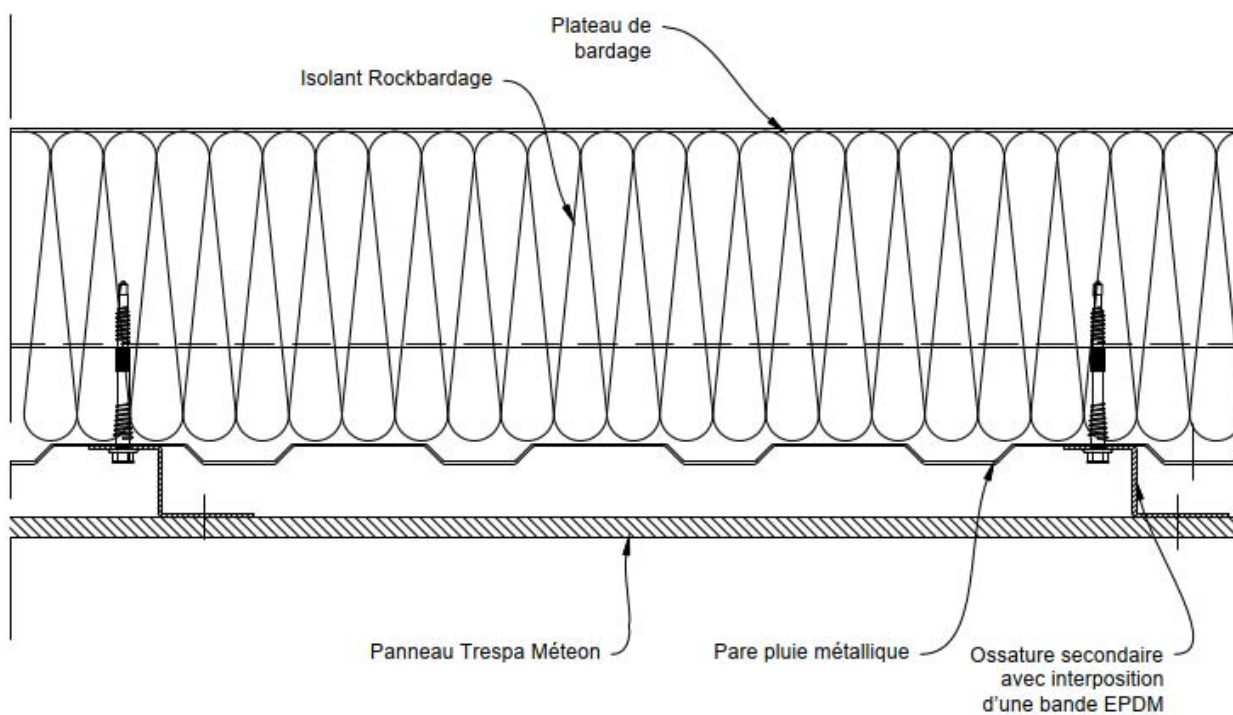
Figure 12 - Joint vertical entre panneaux Trespa® Meteon®.
